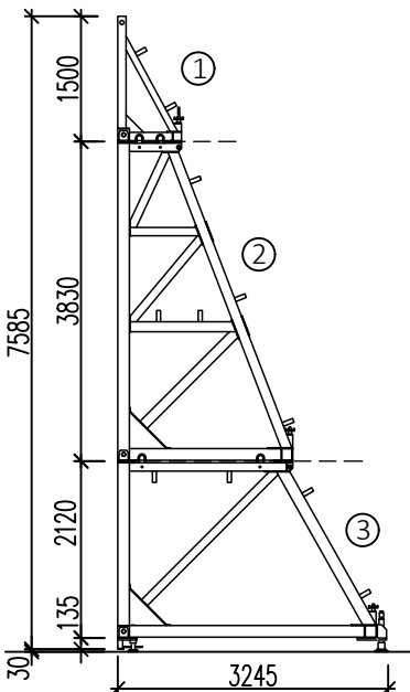
System D: - end piece - support bracket - small extension - front and rear spindle - 3 bolts (weight: 957.0 kg)
