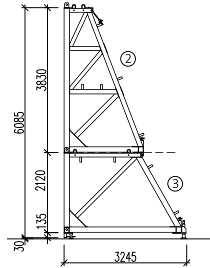
System C: - support bracket - small extension - front and rear spindle - 2 bolts (weight: 881.7 kg)
