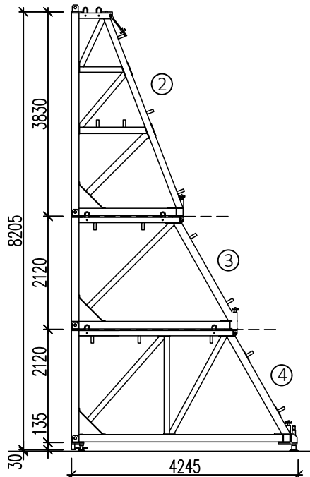
System E: - support bracket - small extension - large extension - front and rear spindle - 3 bolts (weight: 1,362.9 kg)
