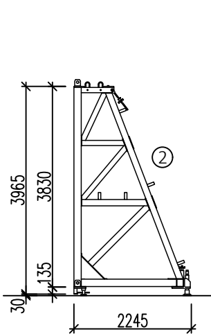
System A: - support bracket - front and rear spindle - 1 bolt (weight: 510.7 kg)
