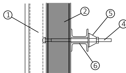
Detail B - Section
