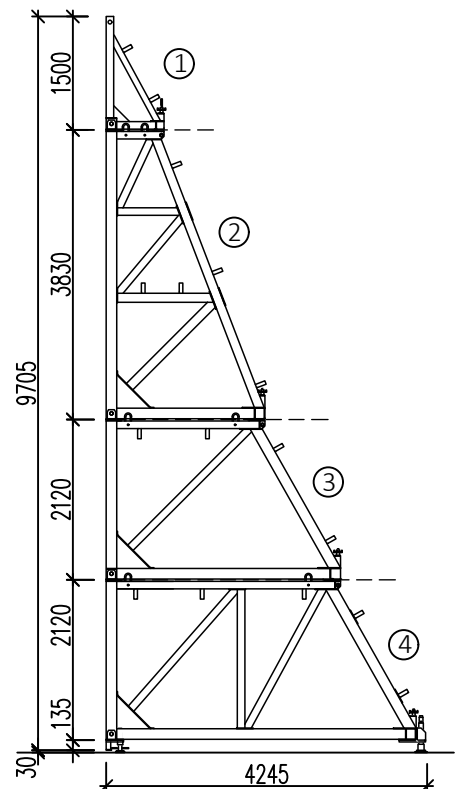
System F: - end piece - support bracket - small extension - large extension - front and rear spindle - 4 bolts (weight: 1,438.2 kg)
